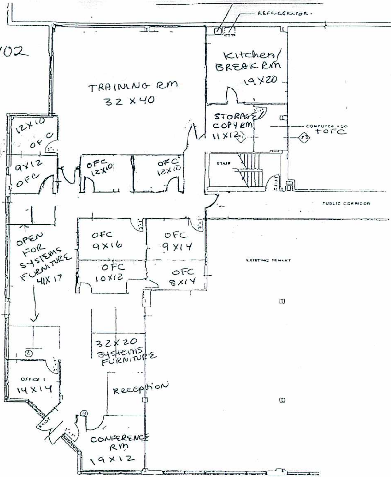
FLOOR PLAN 1/8" = 1'-0"
